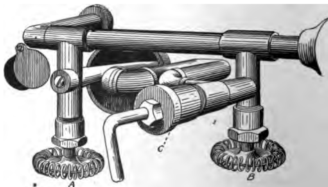
FIG. 367.—Showing the torch in position. By reference to Fig 366, it may be readily understood that the head of the torch, C, is attached to a nipple on B by screw, G; the bent tube being thrust through a port in the burner casing so as to come directly over the fire; the nozzle entering the mixing tube by the side of the nozzle on the main valve, A.
